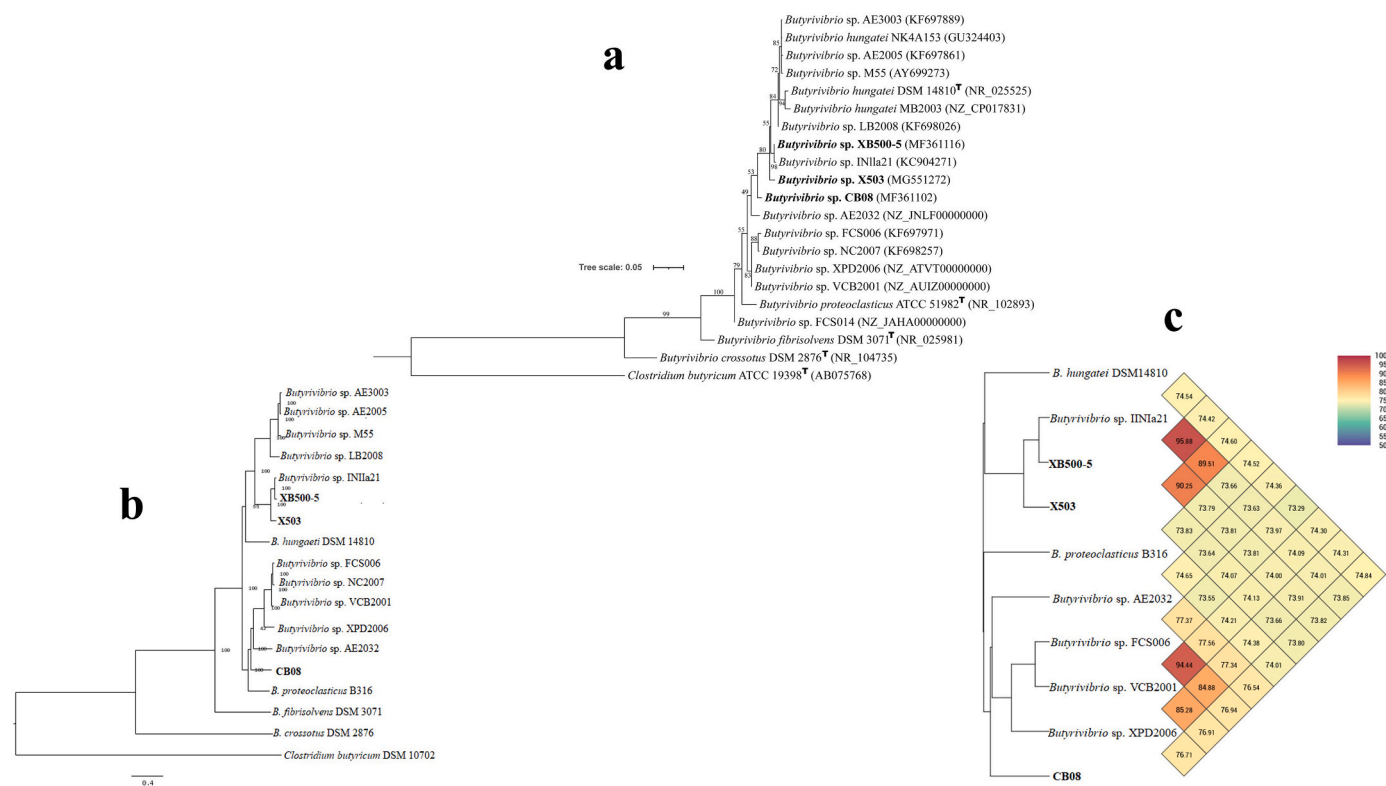
Fig. 1. Phylogenetic tree based on 16S rRNA gene sequences (a) phylogenomic tree (b) codon tree and OrthoANI values (% nucleotide level genomic similarity) tree (c) showing the position of strains CB08, XB500-5 and X503 with other Butyrivibrio strains. (a) The tree was constructed using the Maximum-Likelihood (ML) method on the IQ-TREE web-server. Clostridium butyricum strain ATCC 19398 was used as an outgroup. Bootstrap values based on 1000 replicates are indicated at branching points. The GenBank accession number of each strain is listed in parentheses. Scale bar: 0.05 substitutions per nucleotide position. (b) The tree was generated using the codon tree method within the PATRIC server ( https://patricbrc.org/app/PhylogeneticTree ). A total of 100 single-copy genes found for 16 genomes, and nucleotide sequences were used for each gene. C. butyricum DSM 10702 was used as an outgroup. Bootstrap values based on 500 replicates are indicated at branching points. Scale bar: 0.4 substitutions per nucleotide position.
